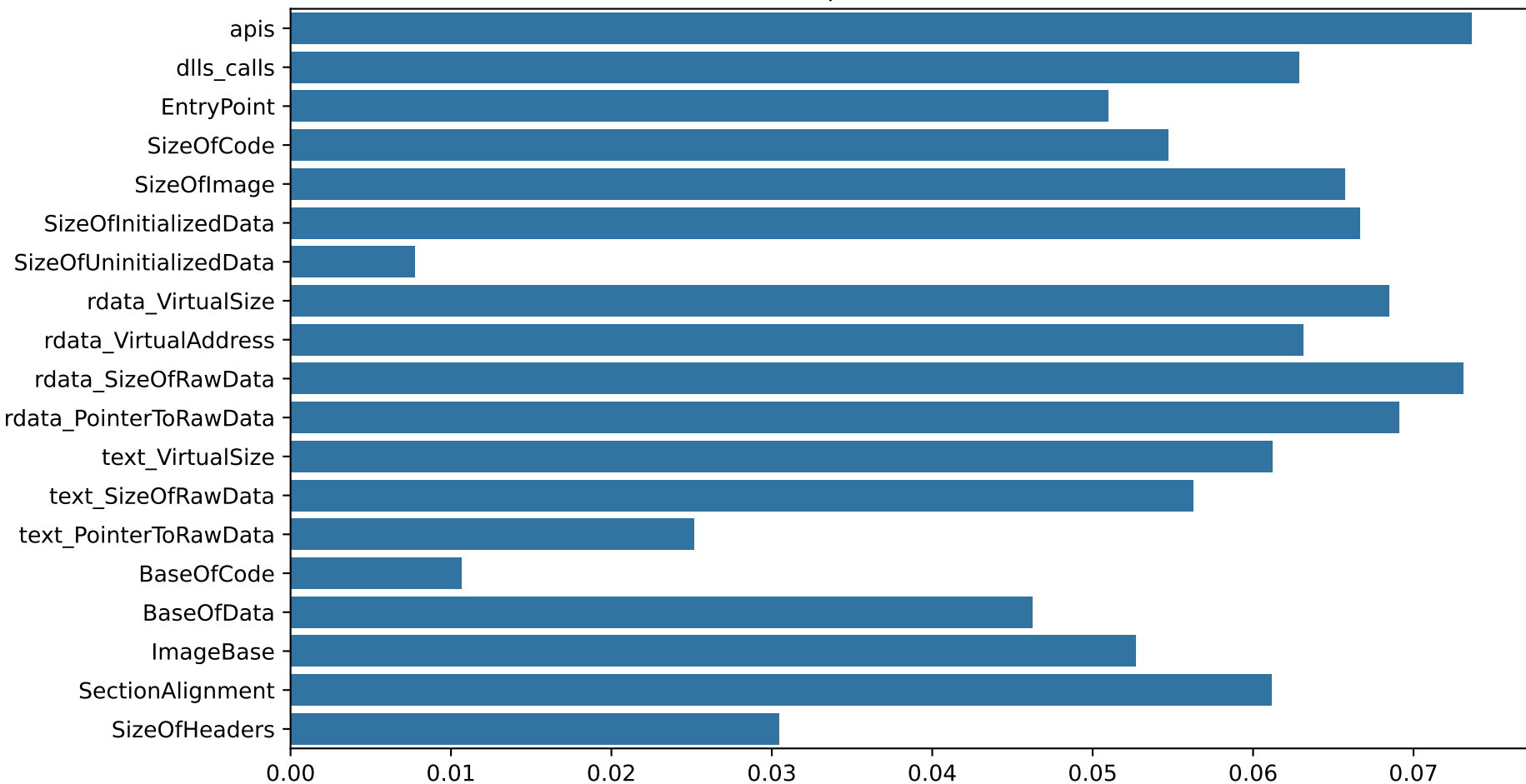
Feature Importances (Extra Trees)
